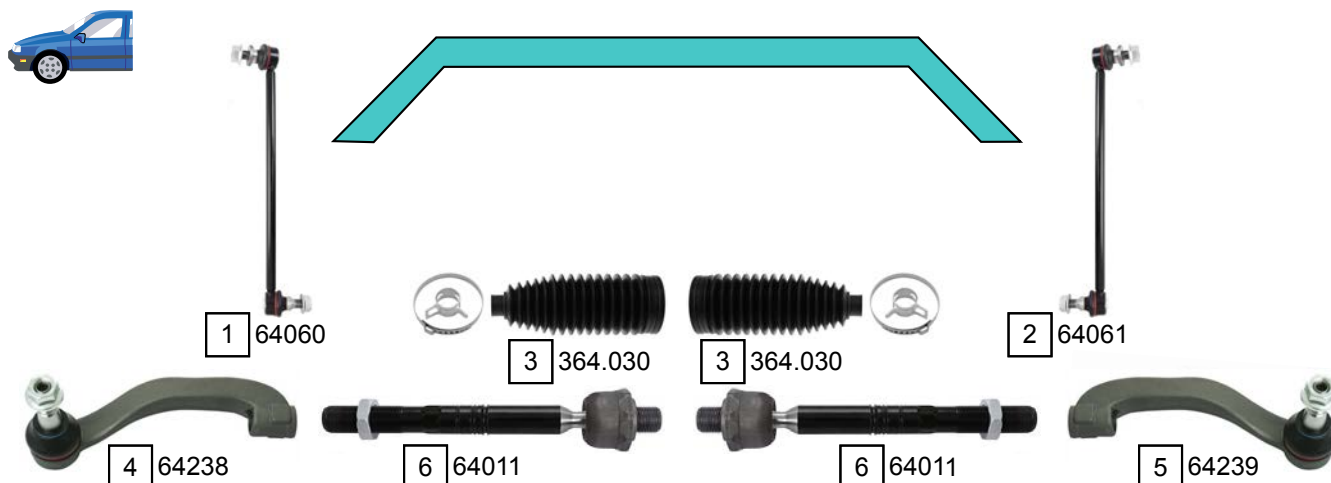
STANDARD FRONT AXLE + BEV
